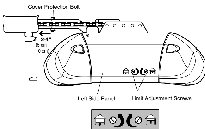
ADJUSTMENT LABEL
