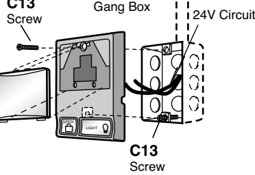
Multi-Function Door Control: Gang Box Installation
